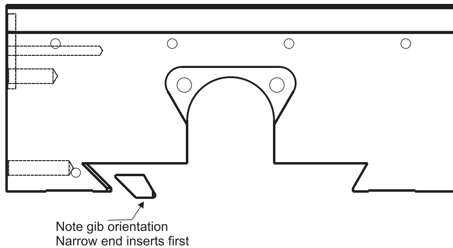
Front View
